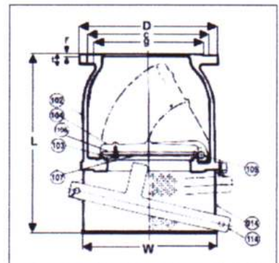
SIZE 200 - 400 mm
