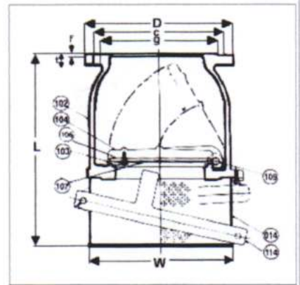
SIZE 200 - 500 mm
