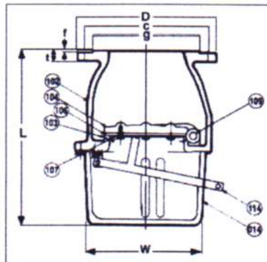
SIZE 65 - 150 mm
