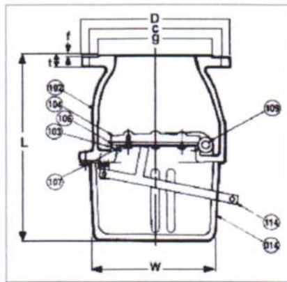
SIZE 65 - 150 mm
