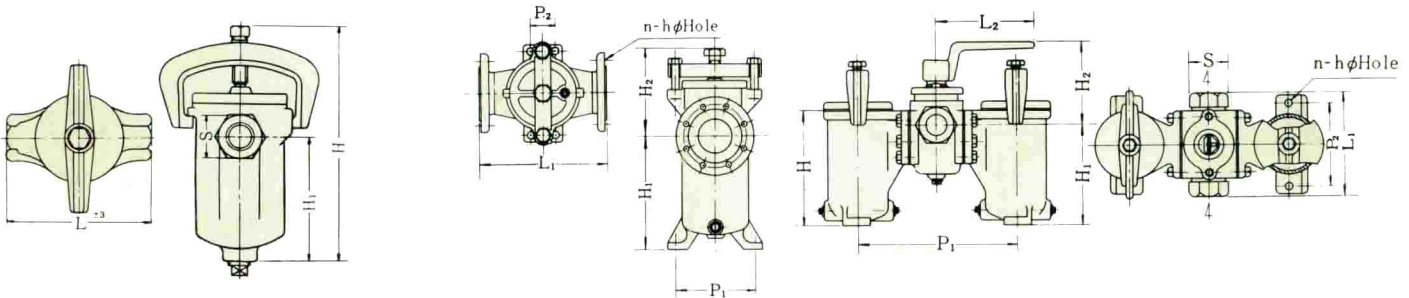
Model STU Single strainer (Size 15—φ40mm)
